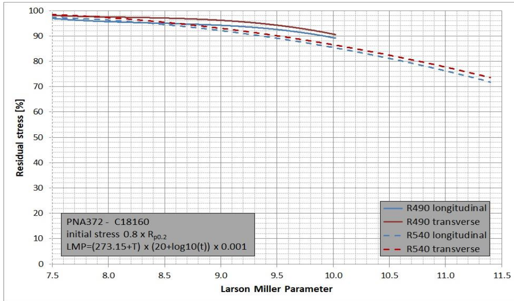
Stress relaxation data of CuCrZr shown as residual stress against Larson Miller Parameter. The Larson Miller Parameter represents temperature and time. Test method: Mandrel test according to ASTM E328.
