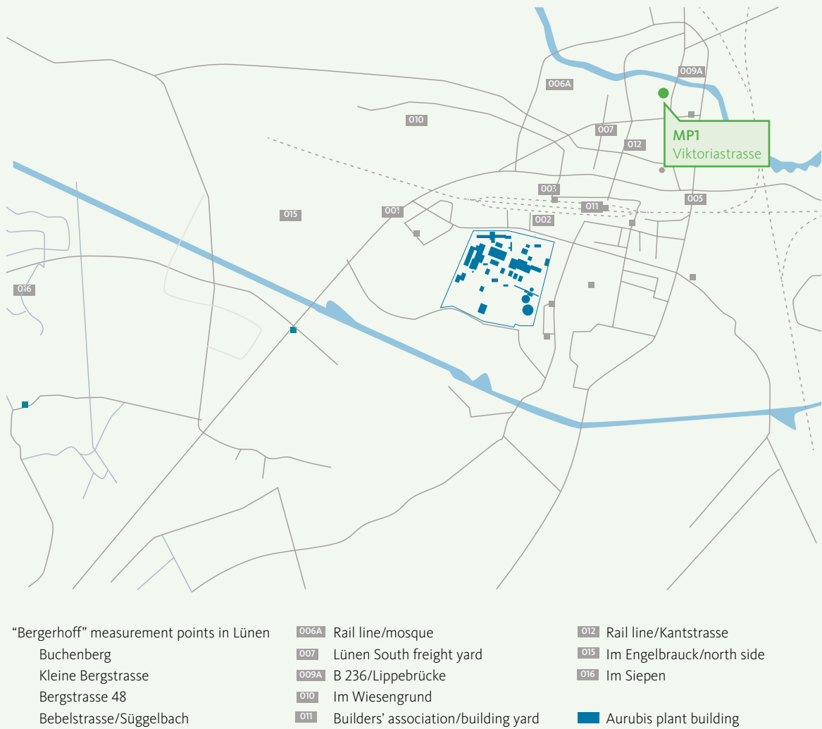
Fig. 3.8: Locations of immission measuring points near the Aurubis plant in Lünen
