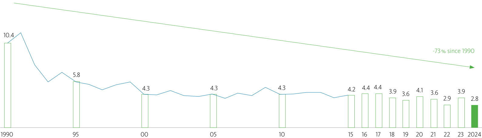
Fig. 2.8: SO 2 emissions at the Hamburg site SO 2 in kg/t of copper output
