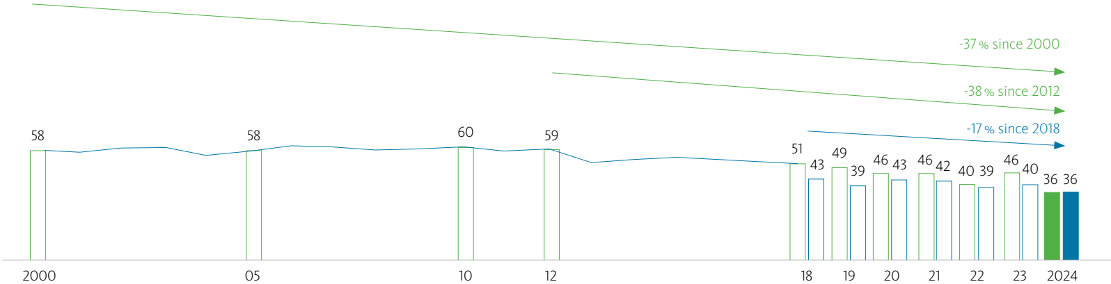
Fig. 1.16: Water withdrawal in Aurubis Group copper production 1 Water withdrawal in m 3 /t of copper output and in g/t of copper equivalent
