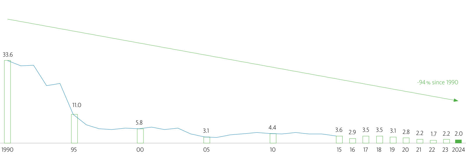
Fig. 2.6: Lead emissions at the Hamburg site Lead in g/t of copper output
