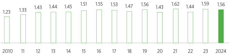
Fig. 3.21: Direct CO 2 emissions at the Lünen site in t CO 2 /t of copper output
