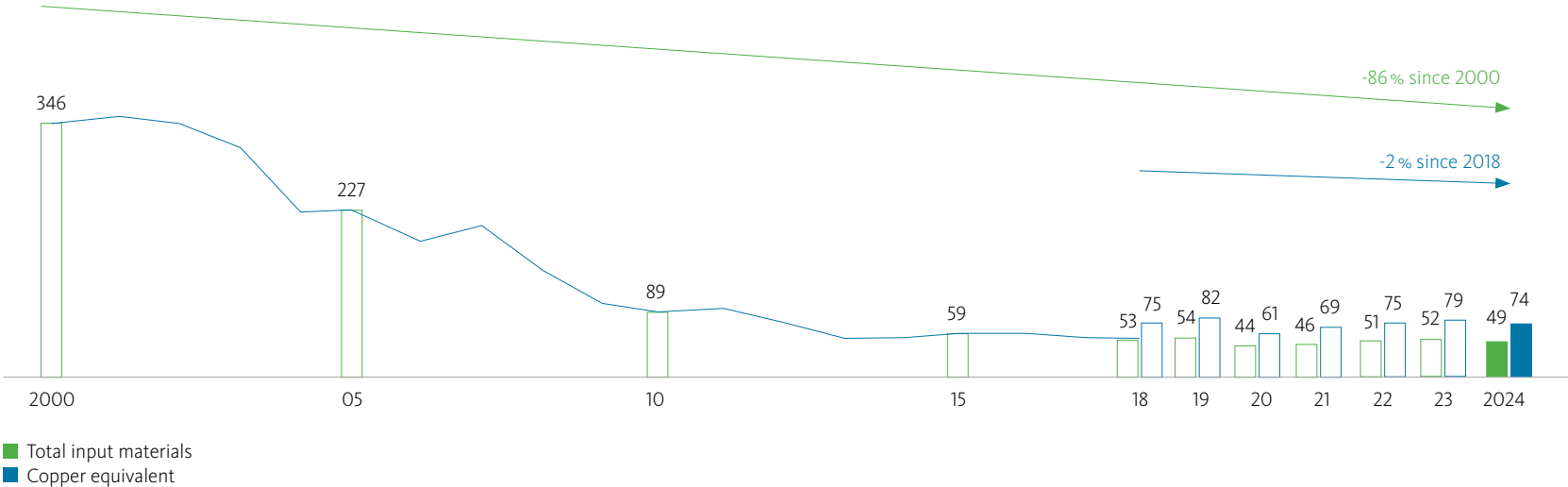
Fig. 3.4: Dust emissions at the Lünen site Dust emissions in g/t of input material and in g/t of copper equivalent
